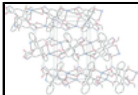
Fig. 3. The hydrogen-bonded (dashed lines) packing in the title compound. H atoms not involved in hydrogen bonding have been omitted for clarity.
