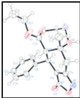
Fig. 1. The molecular structure of the title compound with the atomic numbering scheme. Displacement ellipsoids were drawn at the 30% probability level.
