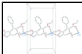
Fig. 2. The polymeric structure of the title compound.
